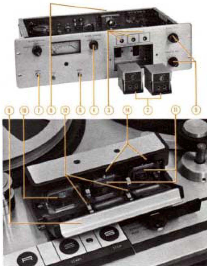
HEAD ASSEMBLY
